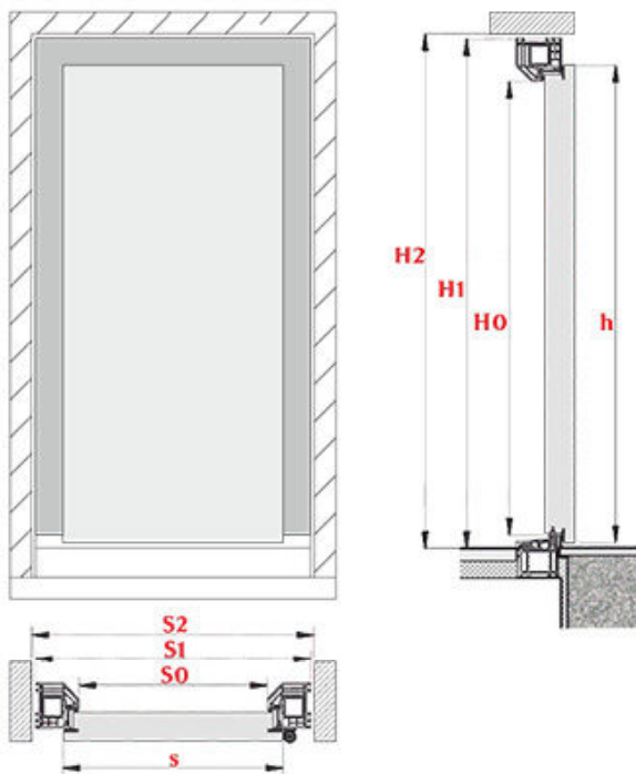
The scheme of door in the rebate version
