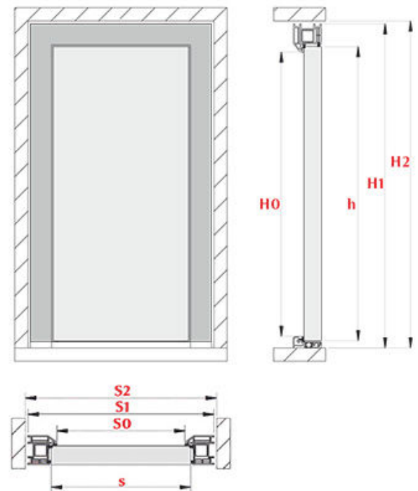
The scheme of door in non-rebated version
